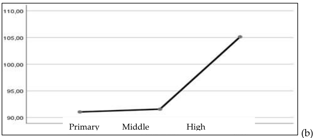
Figure 9: (a) Mathematics anxiety and (b) self-efficacy averages of students according to mother's education level
