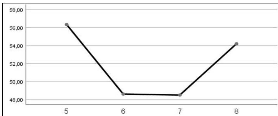
Figure 7: Graph of mathematics anxiety averages of students at grade level
