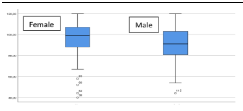
Figure 4: Box chart of the math self-efficacy scale
