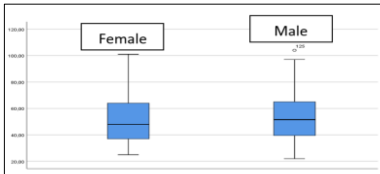
Figure 3: Box chart of the math anxiety scale
