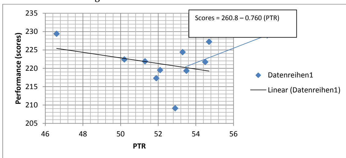
Figure 3.2: Scatter Plot of Test Scores vs. PTR
